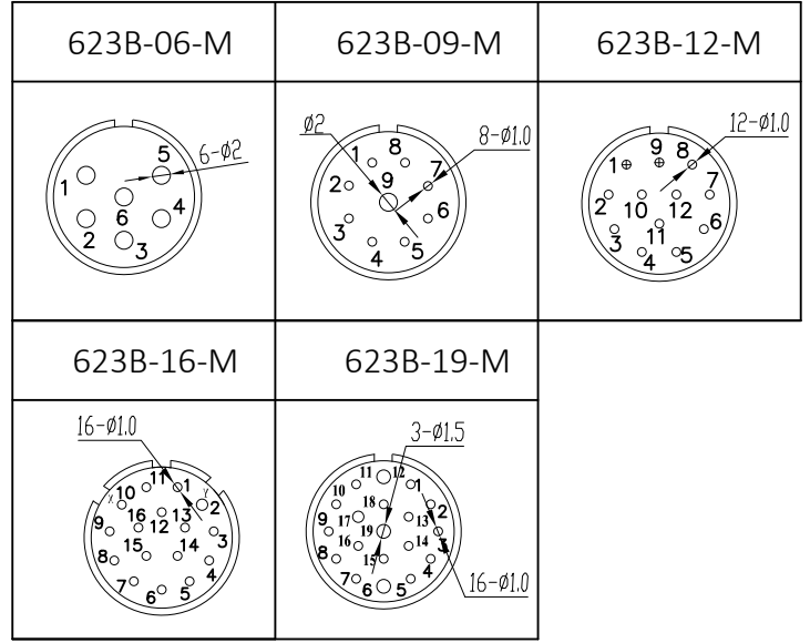
Pin Assignment (Back View)
